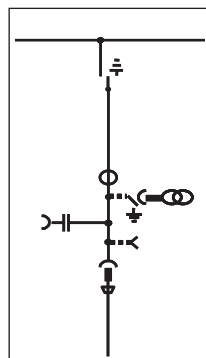
隔离带PT柜
