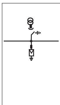
PT避雷器柜
